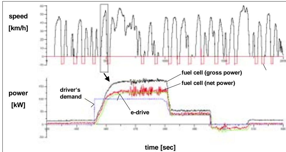
Figure 4: Typical 'power/time' diagram for fuel cell electric drive operation in urban environment [FC-bus in operation in Munich (18 t) - route Obermenzing - Ratzinger Platz]
