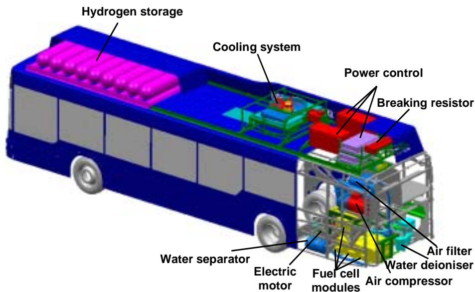
Figure 1: 3-D schematic of the MAN PEM Fuel Cell City Bus
