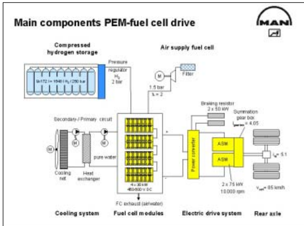
Figure 2: Diagram with main components of the MAN PEMFC city bus
