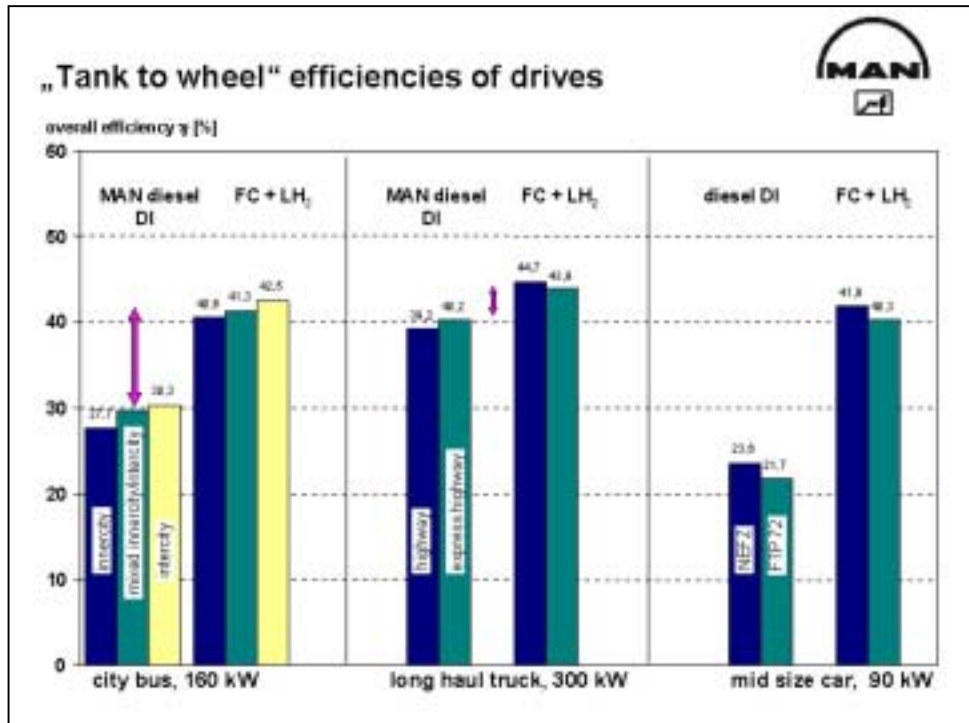
Figure 5: Overall tank-to-wheel efficiencies of PEMFC and Diesel drive systems
