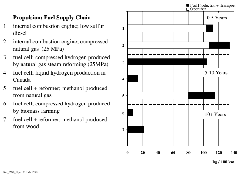
Figure 7: Emissions (in CO 2 -equivalent) of low floor city bus
