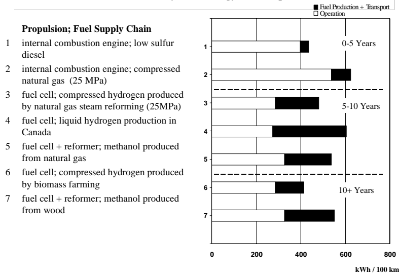
Figure 6: Energy consumption of low floor city bus
