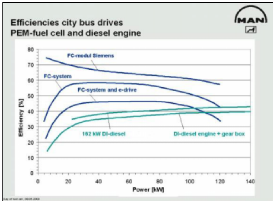
Figure 3: Efficiencies of PEMFC electric drive versus conventional diesel hydraulic drive system
