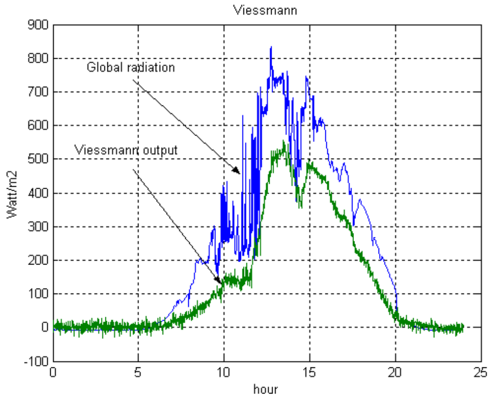
Figure 3: Heat production from Viessman solar collectors
