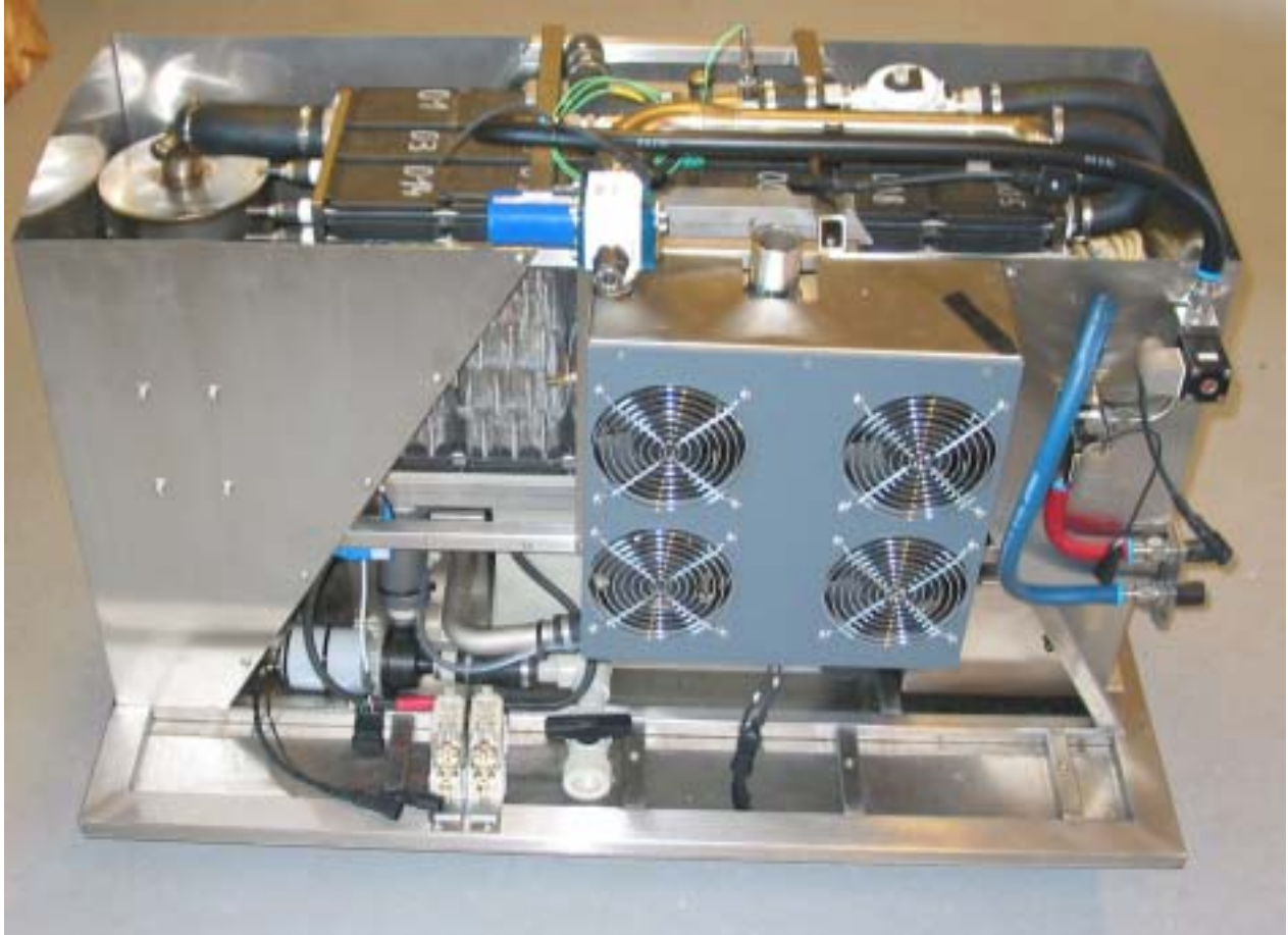
Figure 9: The ZeTek Power fuel cell with electrolyte circulation system, CO 2 removal, etc.
