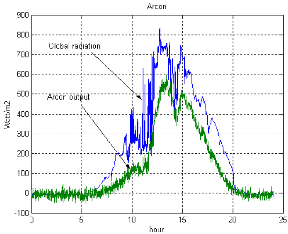
Figure 4: Heat production from Arcon solar collectors
