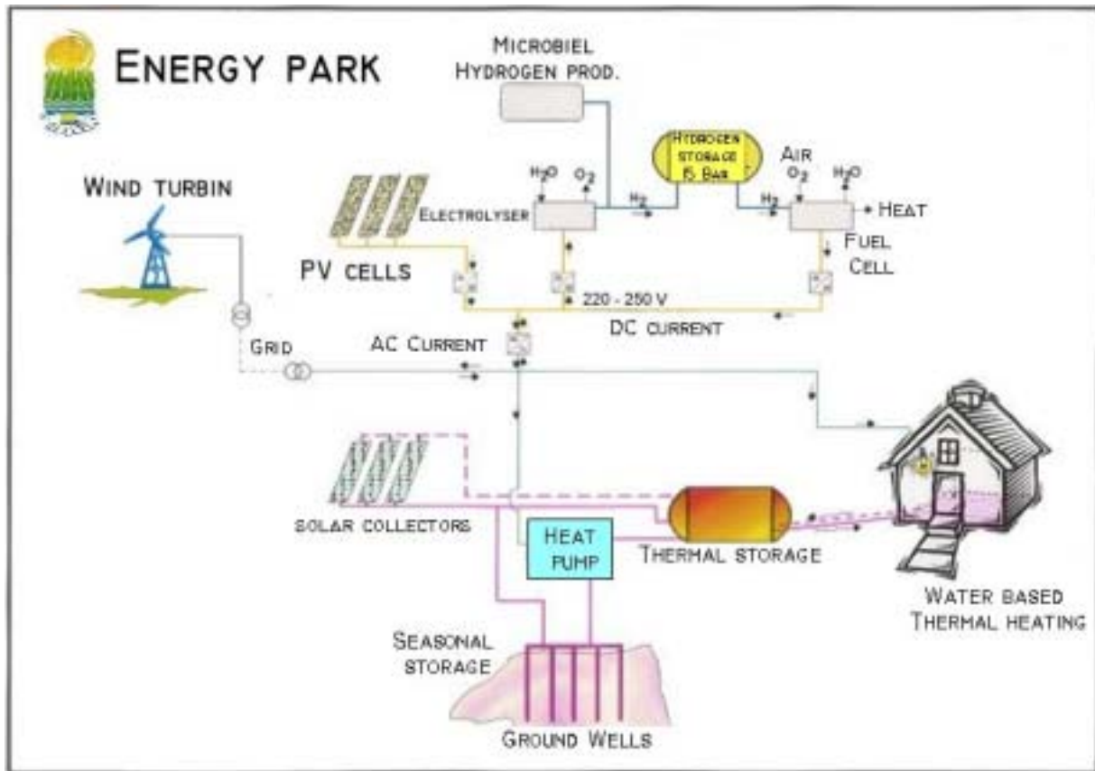
Figure 2: A schematic drawing of the Energy Park
