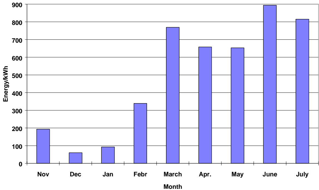
Figure 14: The electrical energy delivered to the grid from November 2001 to July 2002
