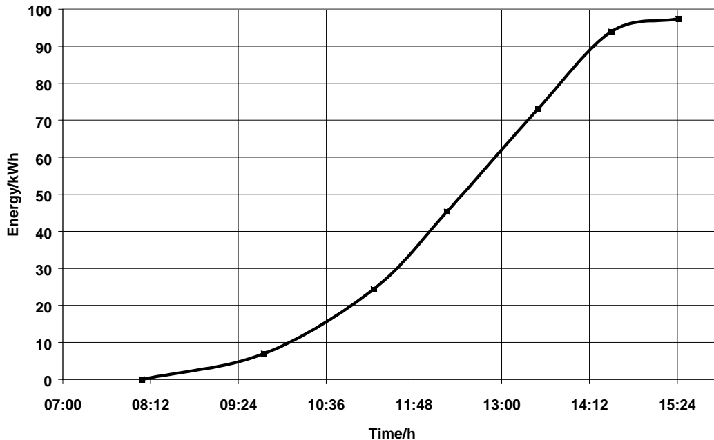
Figure 15: Cumulative thermal energy production on a sunny day in November 2001
