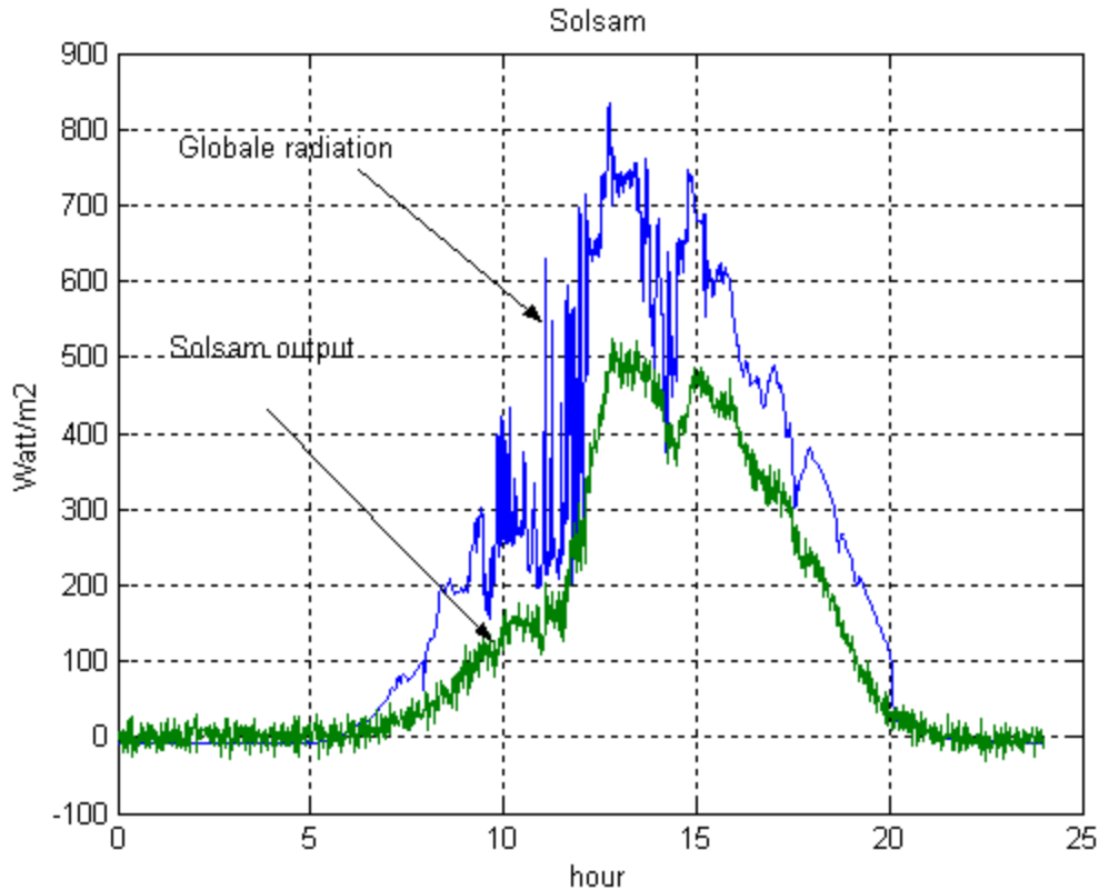
Figure 5: Heat production from Solsam solar collectors
