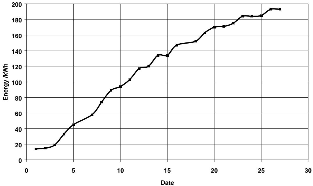
Figure 13: Cumulative electrical energy delivered to the grid in November 2001
