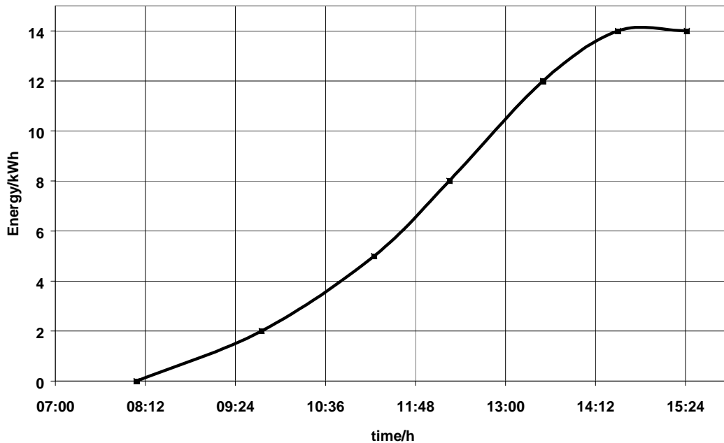
Figure 12: Cumulative electrical energy delivered to the grid on a sunny day in November 2001
