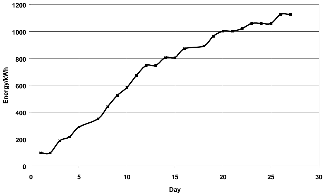
Figure 16: Cumulative thermal energy produced in November 2001
