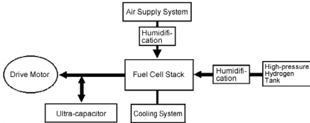
Figure 3: System outline diagram
