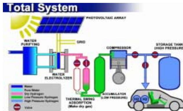
Figure 2: Schematic of Honda's hydrogen fueling station
