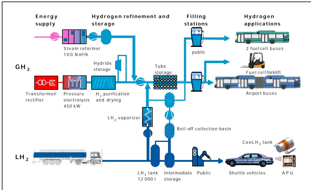
Figure 1: Overview of the hydrogen project at Munich International Airport
