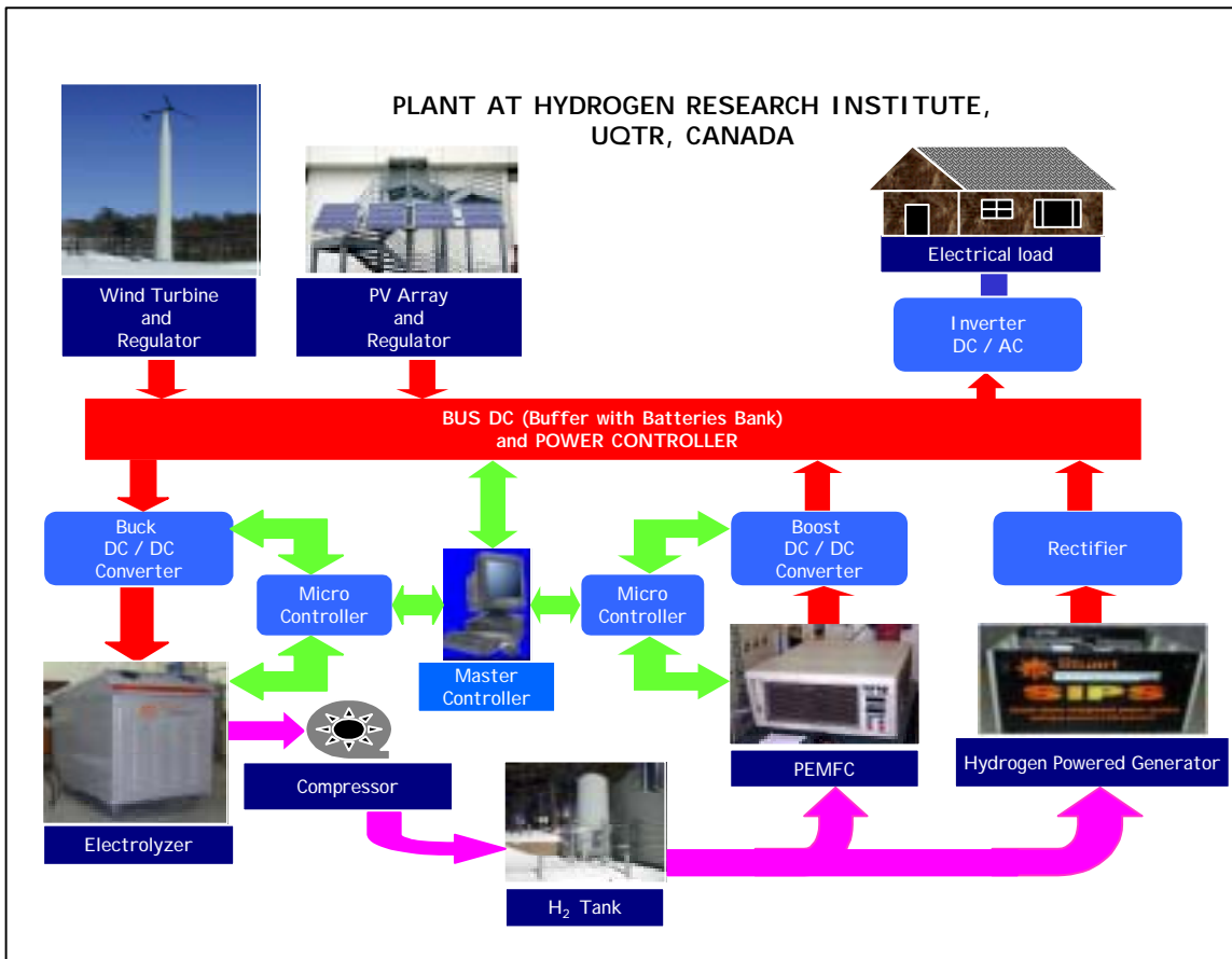
Figure 1: Stand-alone Renewable Energy System at the Hydrogen Research Institute
