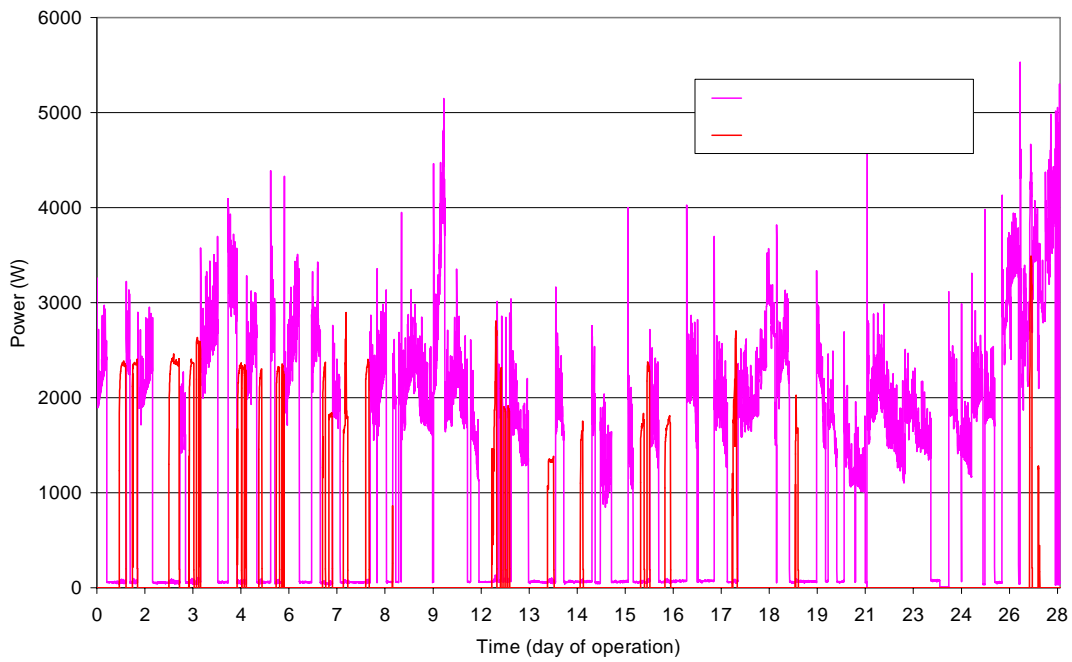
Figure 5: Electrolyser input and fuel cell output
