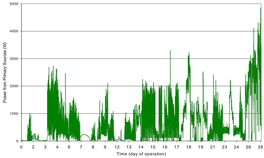
Figure 4: Power available from primary energy sources
