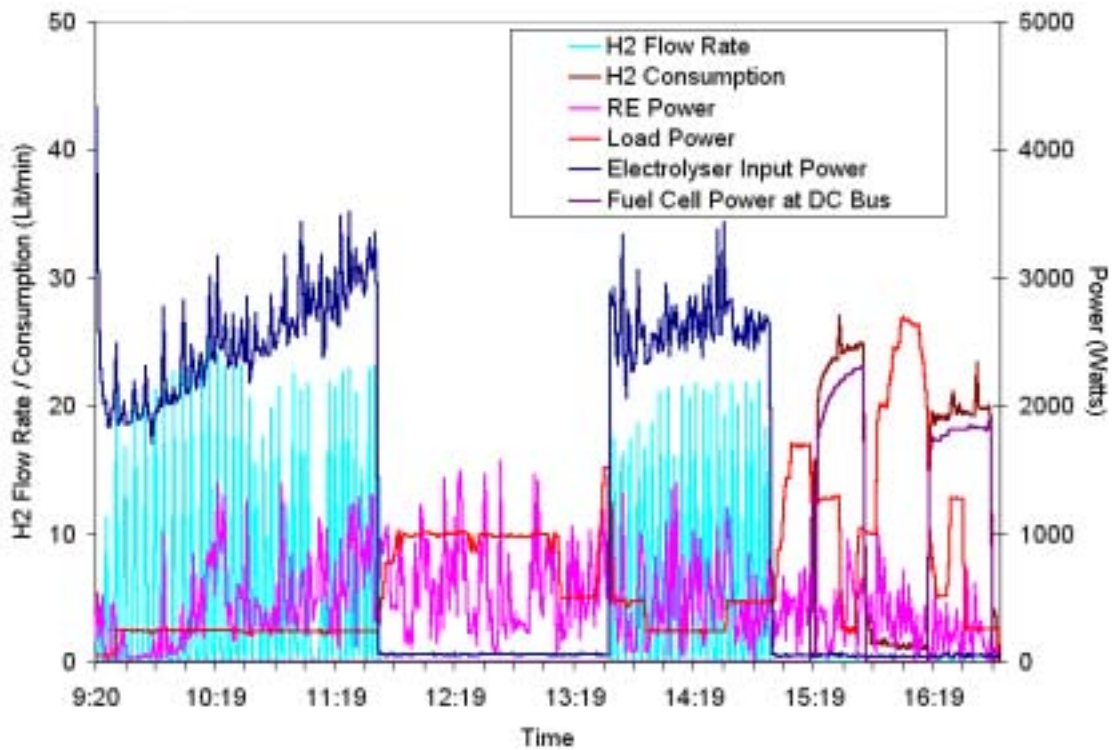
Figure 3: Power, H 2 flow rate and consumption rate in RE system on Dec 10, 2001
