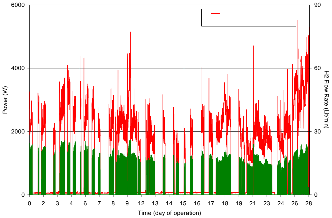
Figure 7: Electrolyser input power and H 2 flow rate
