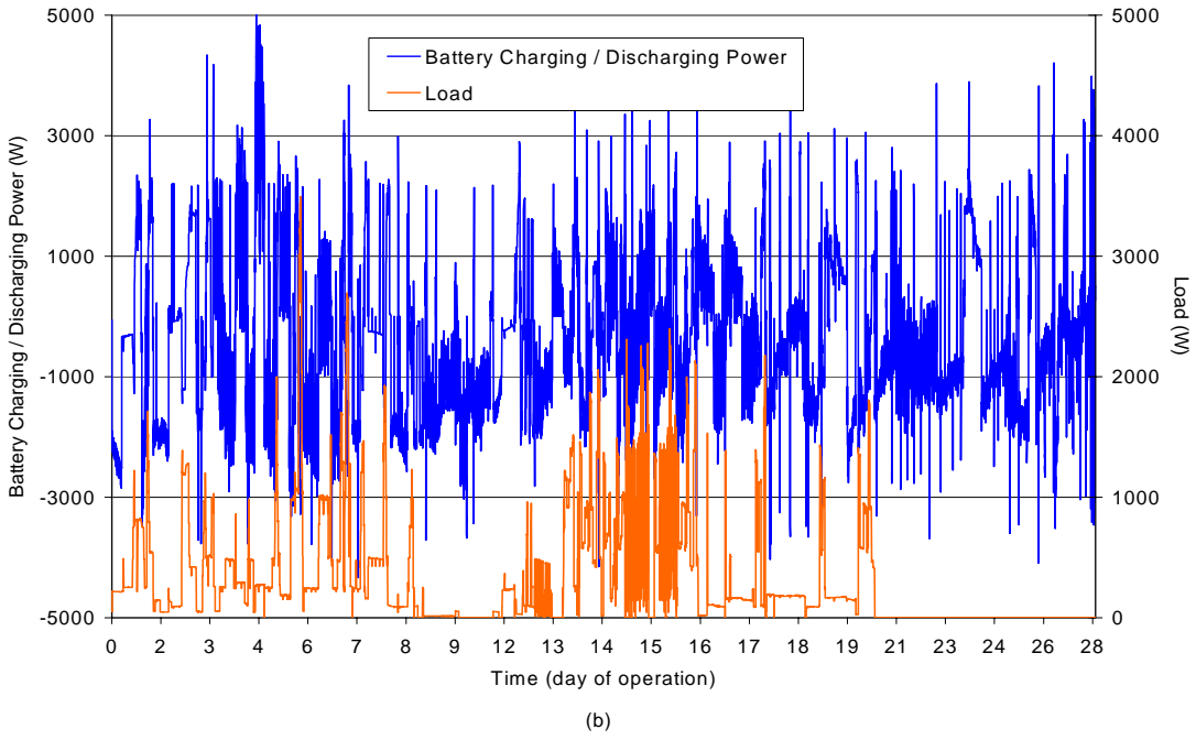
Figure 6: Battery charging /discharging and load power
