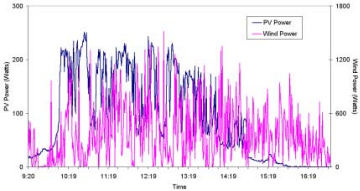
Figure 2: Power available from wind turbine generator and PV array on Dec 10, 2001
