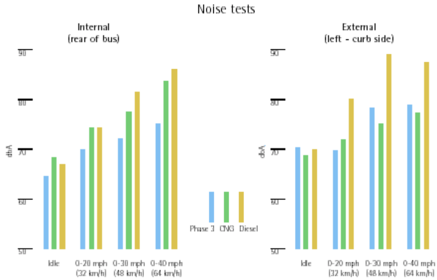
Figure 12: Noise tests
