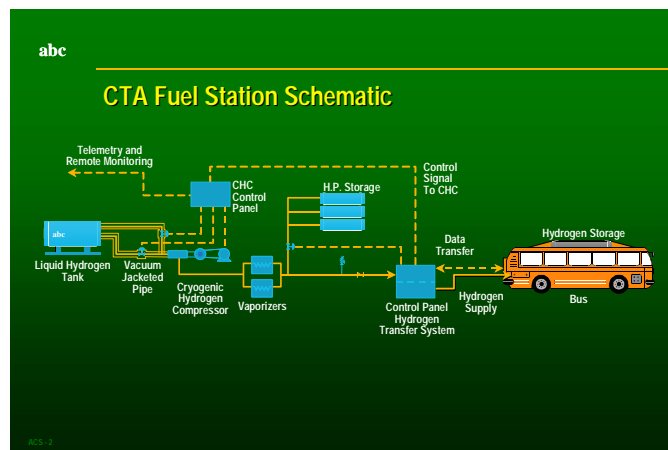
Figure 6: Schematic of the CTA hydrogen fueling facility
