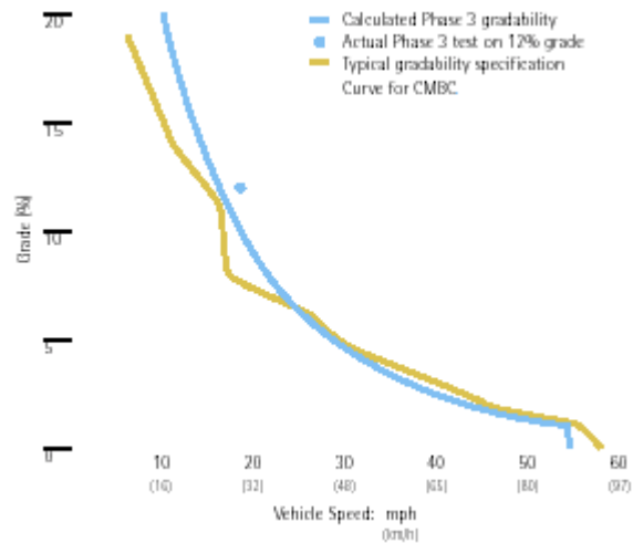
Figure 11: Typical gradability at 17 tons (15.4 tonnes)
