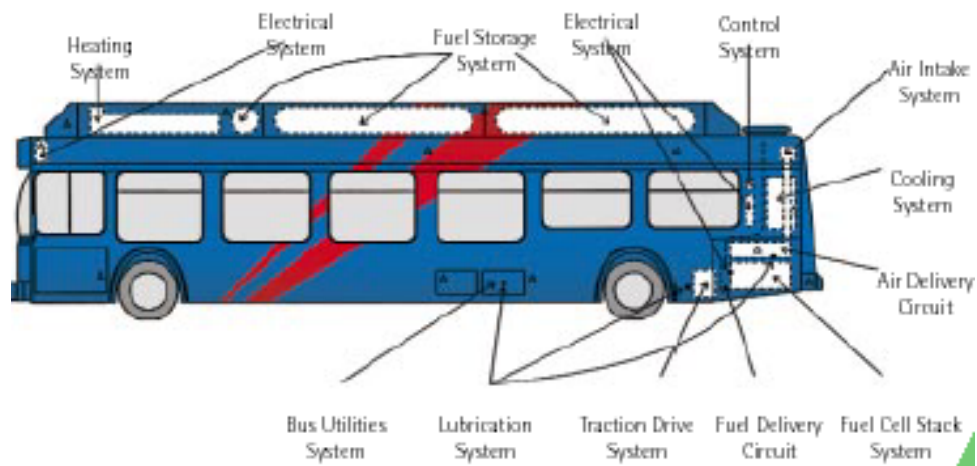
Figure 2: Schematic picture of XCELLSIS/Ballard fuel cell bus
