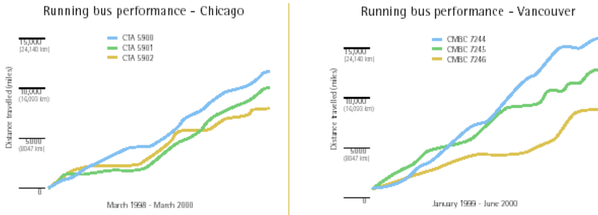
Figure 13: Running bus performance in Chicago and in Vancouver
