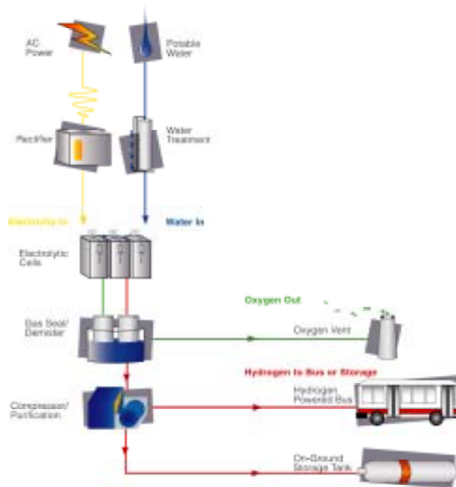
Figure 8: Process flow of fuel appliance
